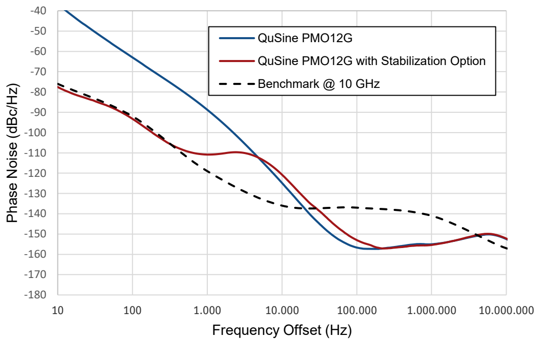
Measured SSB Phase Noise at 12 GHz
